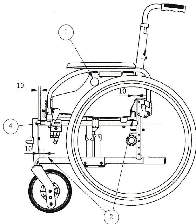
Left View
